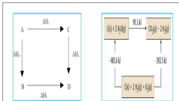
Figure 1a. Hess Law Process
