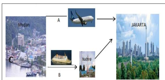
Figure 1b. Hess Law Analogy
